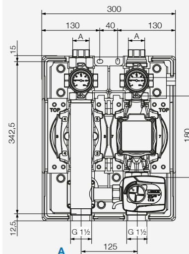
FLOWBOX HKM25/32
