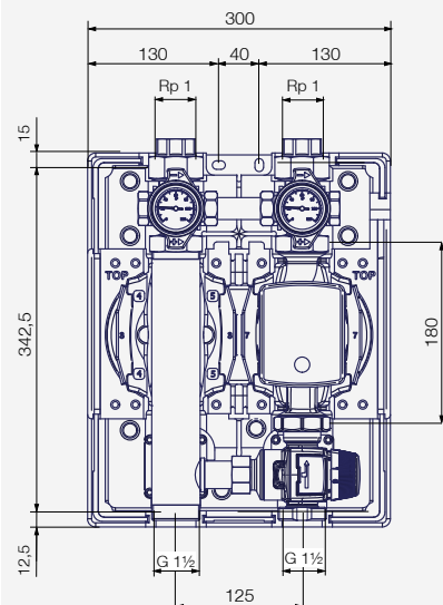
FLOWBOX HKF25
