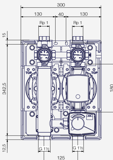
FLOWBOX HKFC25
