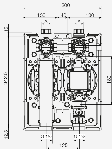
FLOWBOX HK25-KH
