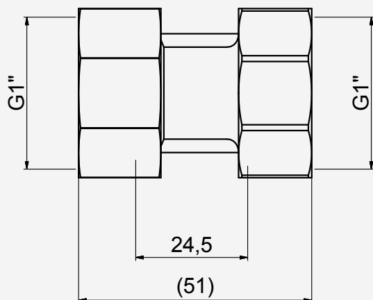
KUPPLUNG 1"
